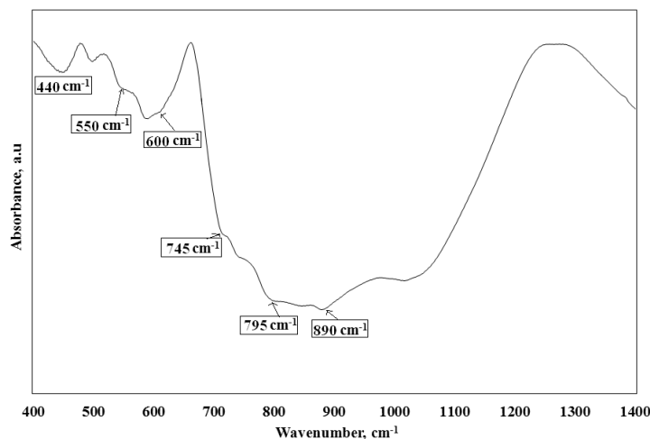
Fig. 5. The FTIR spectra of as-quenched 65\text{GeO}_2\text{-}15\text{PbO}\cdot 10\text{MgO}\cdot 10\text{MgF}_2 sample after annealing at 800\text{ }^\circ\text{C} for 60 minutes.
