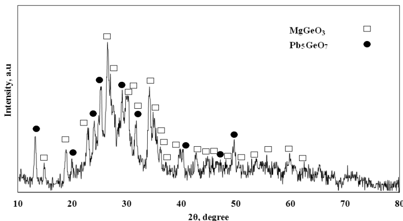
Fig. 4. The XRD pattern of as-quenched 65\text{GeO}_2\text{-}15\text{PbO}\cdot 10\text{MgO}\cdot 10\text{MgF}_2 sample after annealing at 800\text{ }^\circ\text{C} for 60 minutes.
