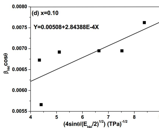
Figure 6(a-d). The plots \beta_{hkl}\cos\theta Vs 4\sin\theta(2/E_{hkl})^{1/2} of Zn_{1-x}Mn_xO
