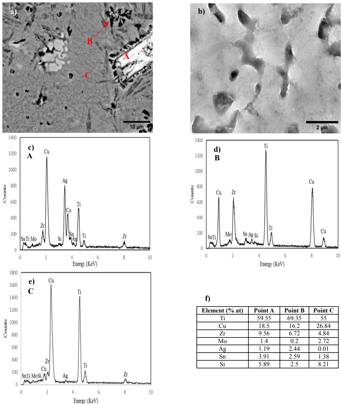
Fig. 2. Electron microscope image of different alloys a) Ti_{50}Zr_{15}Cu_{20}Mo_7Ag_4Sn_3Si_1 and b) Ti_{50}Zr_{25}Cu_5Mo_{10}Ag_6Sn_3Si_1 , c-f) EDS analysis of different areas in the Ti_{50}Zr_{15}Cu_{20}Mo_7Ag_4Sn_3Si_1 alloy
