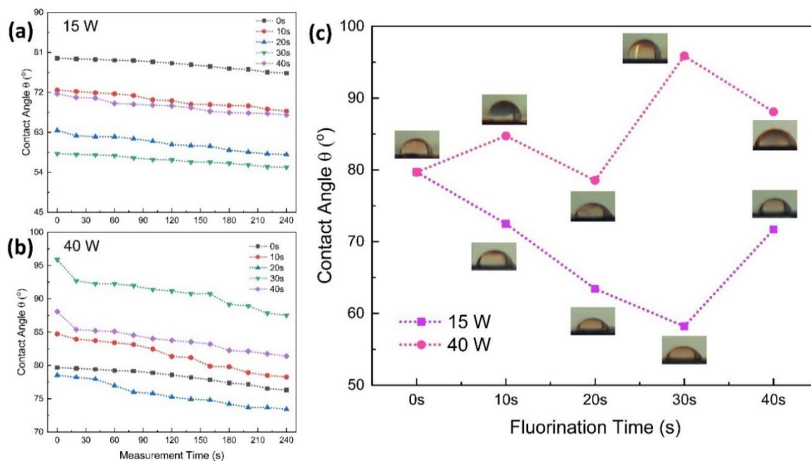
Fig. 3. Water contact angle measurement results on of 0 s-40 s fluorinated graphene at a) 15 W and b) 40 W SF 6 plasma in 240 s measurement time, c) comparison of contact angles at 0 s-40 s fluorination time in a single measurement time
