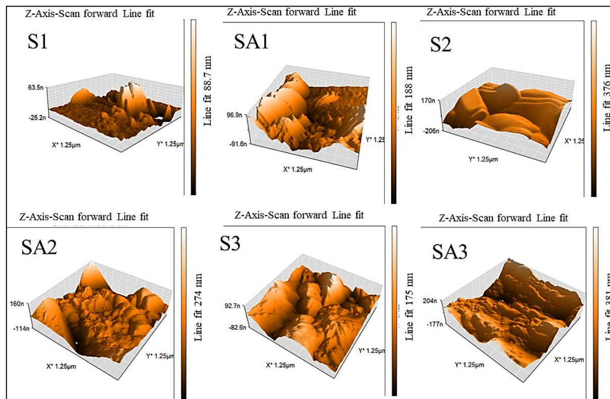
Fig. 9. Three-dimensional AFM images for pure and Cu doped CdO x samples deposited at room temperature and annealed at 450 °C
