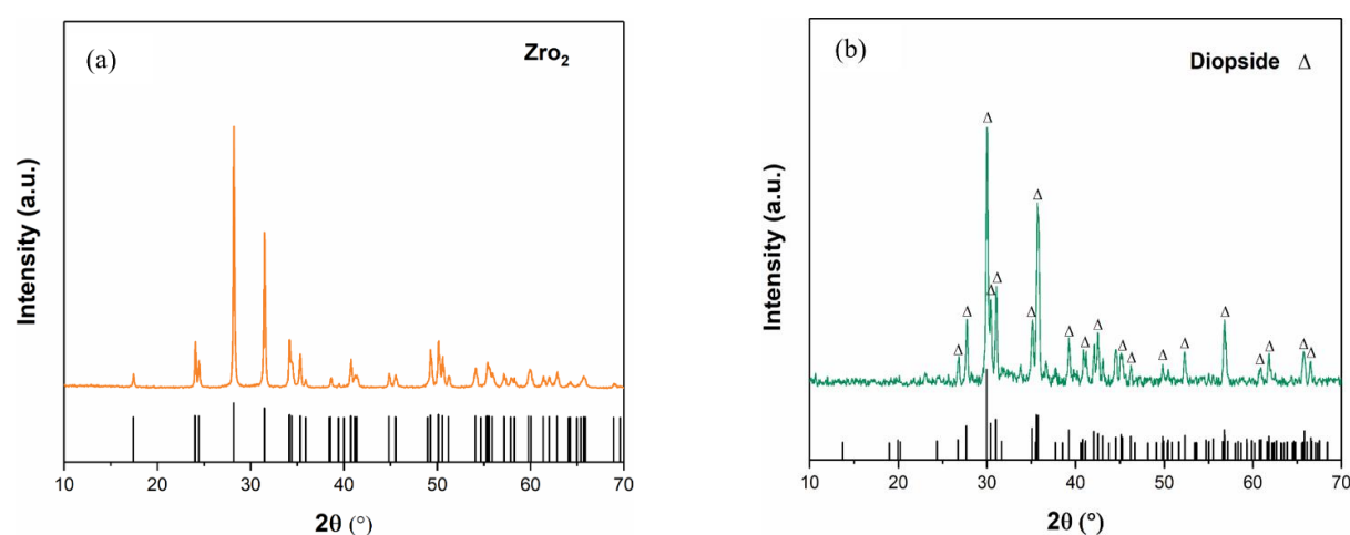
Fig. 2. XRD patterns of a) purchased zirconia ( ZrO_2 ) and b) synthesized diopside ( CaMgSi_2O_6 )
