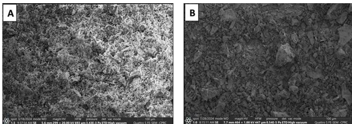
Fig. 2. SEM A, Study Amber resultant fine powder (12.275 μm); and B, VITA Lumex® AC powder (26.672 μm)
