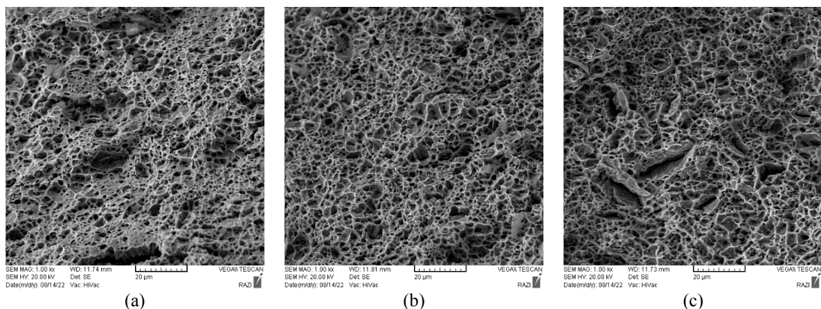
Fig. 12. Fractography of tensile failure samples a) GTAW 25% CW and b) GTAW 50% CW c) PCGTAW 50% CW
