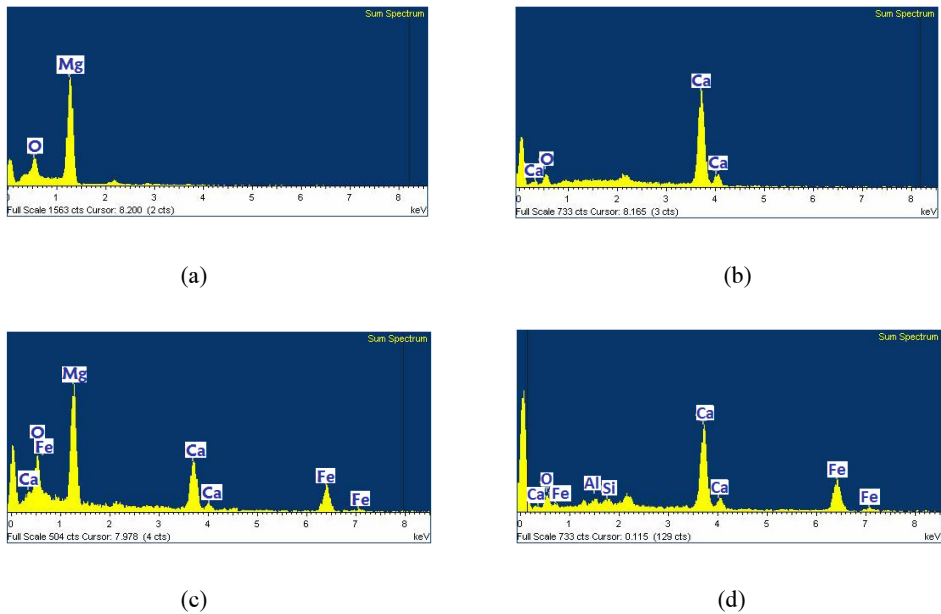
Fig. 5. EDS analyses of Fig. 4-b: (a) region P (periclase grain), (b) region L (Lime grain), (c) region MF (Magnesioferrite precipitates) (d) region GB (grain boundaries)
