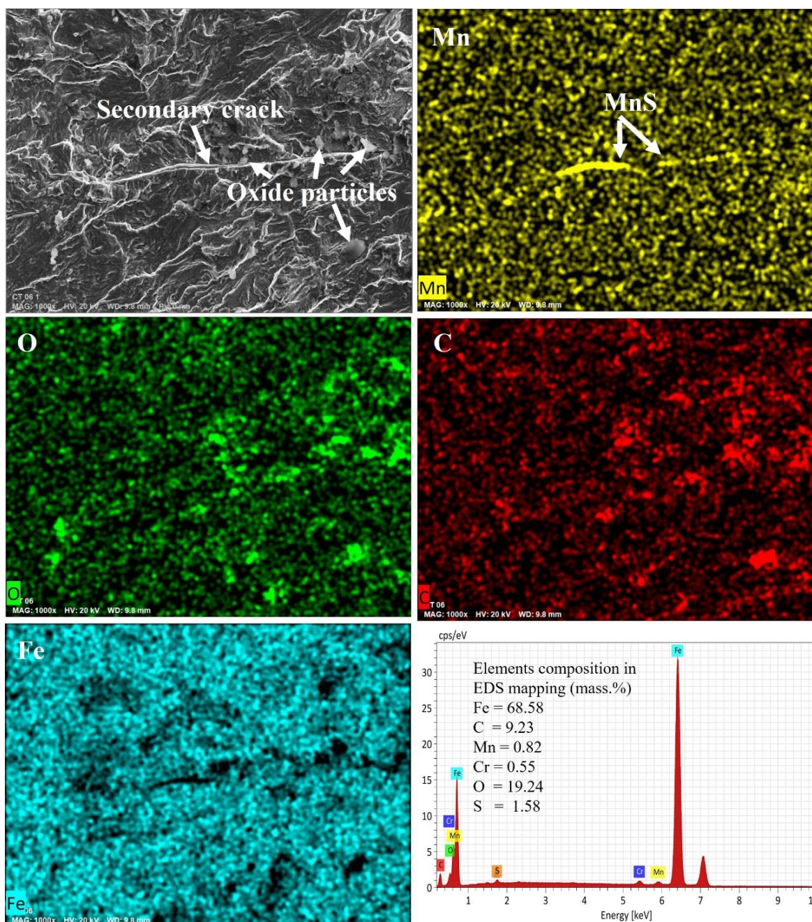
Fig. 9. SEM fractographic surface of the LT specimen observed at a crack length of approximately 0.3 mm, showing the elemental mapping of Mn, O, C, Fe, and the corresponding EDS spectra
