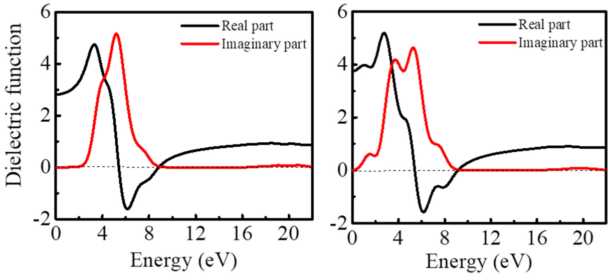
(a) \text{SrTi}_{0.875}\text{Cr}_{0.125}\text{O}_3
