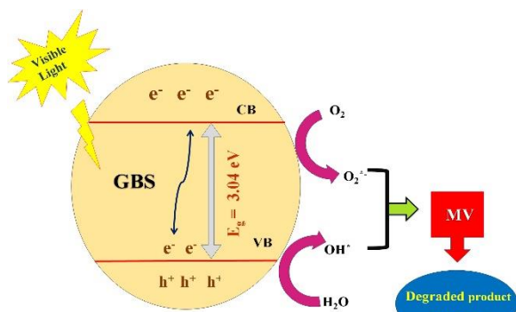
Fig. 14. Photocatalytic mechanism involved with GBS catalyst
