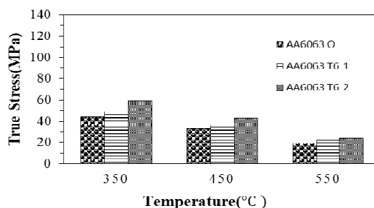
Fig. 14. The effects of heat treatment of AA6063 alloy on the flow stress at ε=0.5.
