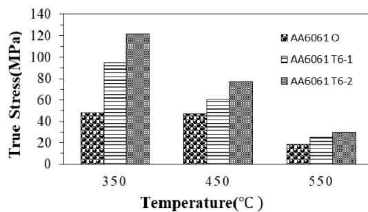
Fig. 13. The effects of heat treatment of AA6061 alloy on the flow stress at ε=0.5.
